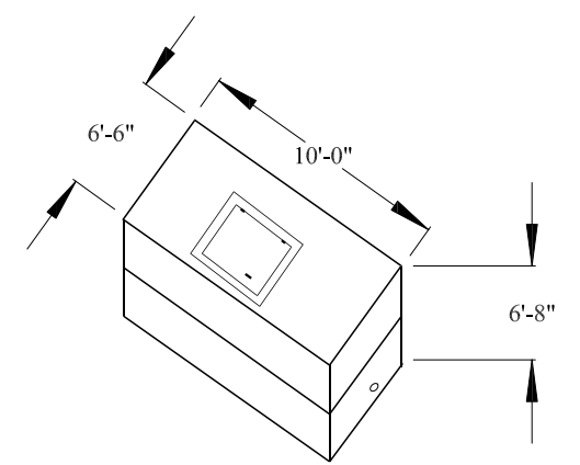
ASSEMBLED TANK
