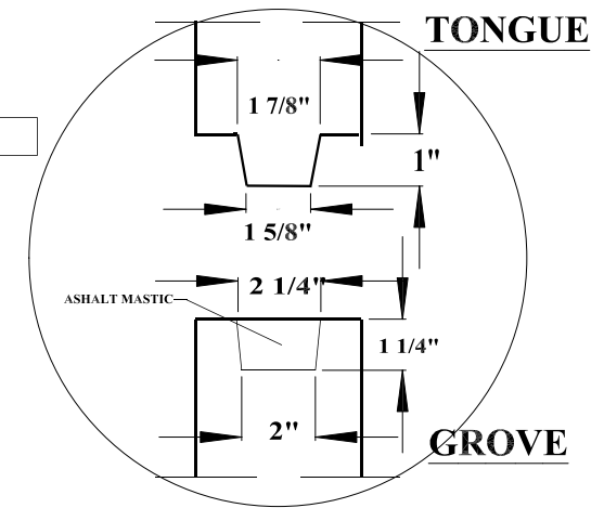
JOINT DETAIL
